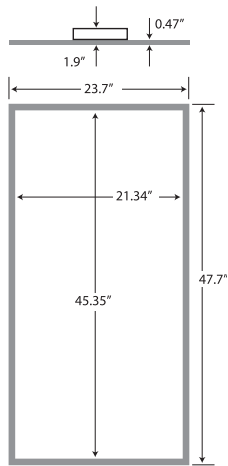
52W 2x4 LED Panel
