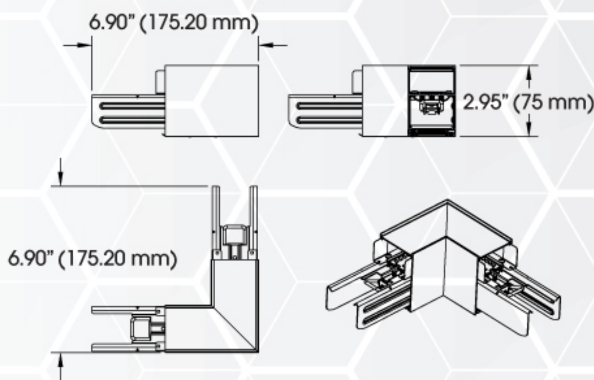
L-CONN
