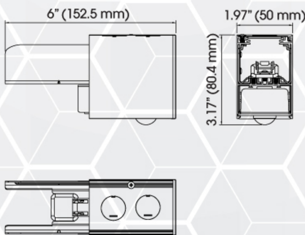
END CAP W/SENSOR
