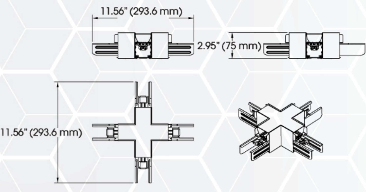
X-CONN
