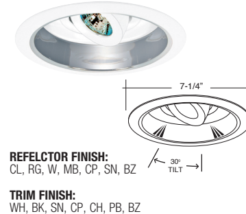
B1619W-WH ADJUSTABLE SPOT (30° TILT)
