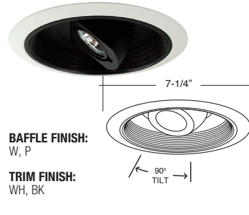
B1621P-WH ADJUSTABLE SPOT (90° TILT)
