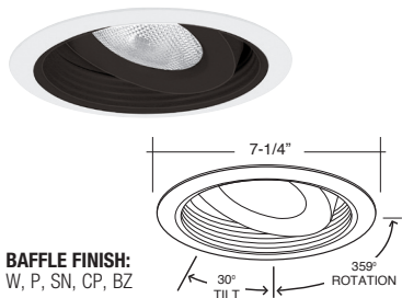
B1673P-WH PAR36 BAFFLE WITH GIMBAL RING
