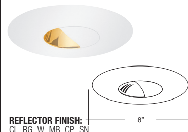
B1644RG-WH REFLECTOR WALL WASH
