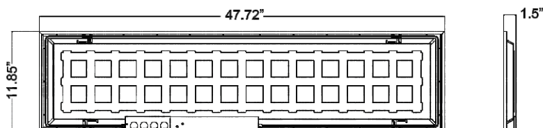
PLB14 Dimensions mm | 1212 (L) x 301(W) x 38(H) inch | 47.72(L) x 11.85(W) x 1.5(H)
