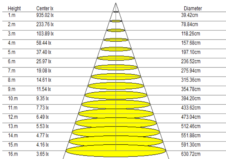
Lux Distance Curve Beam angle: 22.30° (50% Imax)
