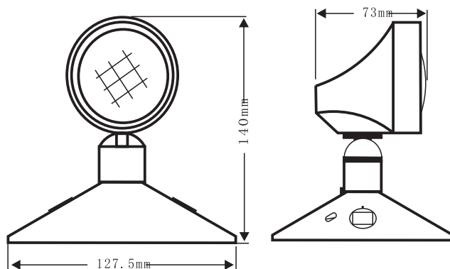
CM201A Dimensions mm | 128(Ø) x 140(H) inch | 5(Ø) x 5.5(H)
