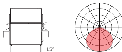
1.5" Drop Lens
