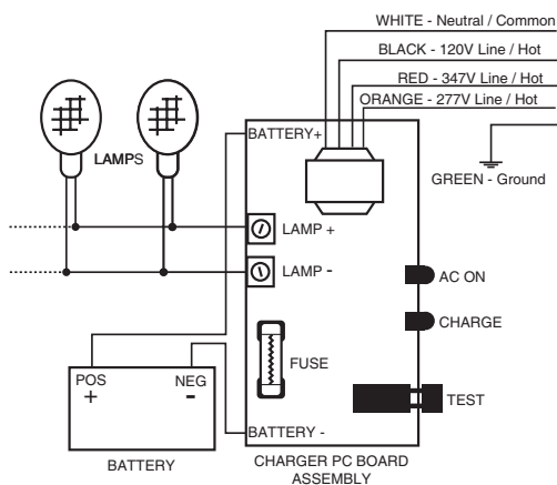
CHARGER BOARD STANDARD DUAL INPUT VERSION
