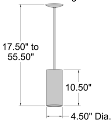
Line Drawing #1
